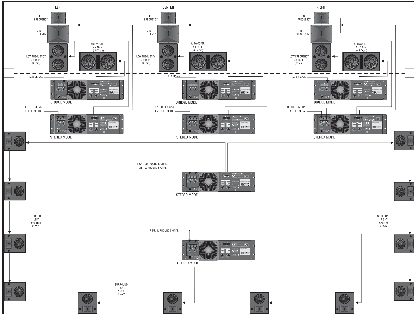
Figure 3.14 Typical Large 3-Way System (CE 2000TX Amplifiers Shown with Optional CEAS1 Output Module)
