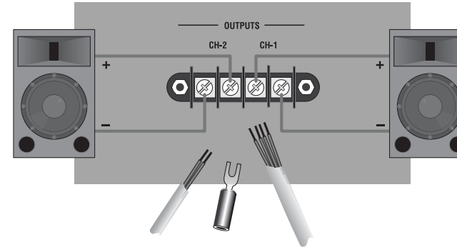
Figure 3.7 Output Connector Wiring for Stereo with Optional CEAS1 Output Module.
