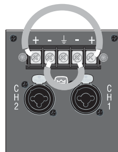
Figure 3.10 Placement of Jumpers to Parallel the Inputs
