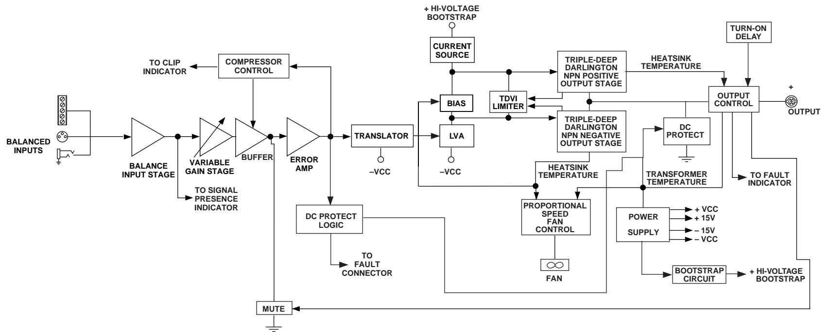
Figure 6.1 CE 2000TX Amplifier Block Diagram (Shown with Standard Input Module)
