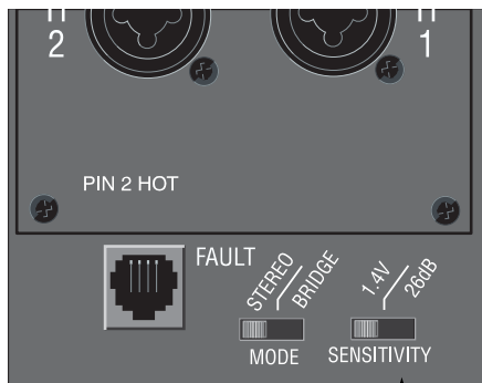
Sensitivity Switch
