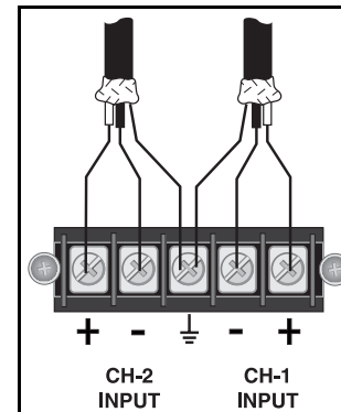
Figure 3.5 Barrier Strip Input Wiring: Balanced Signal In
