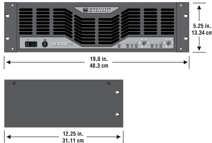
Figure 3.1 CE 2000TX Dimensions
