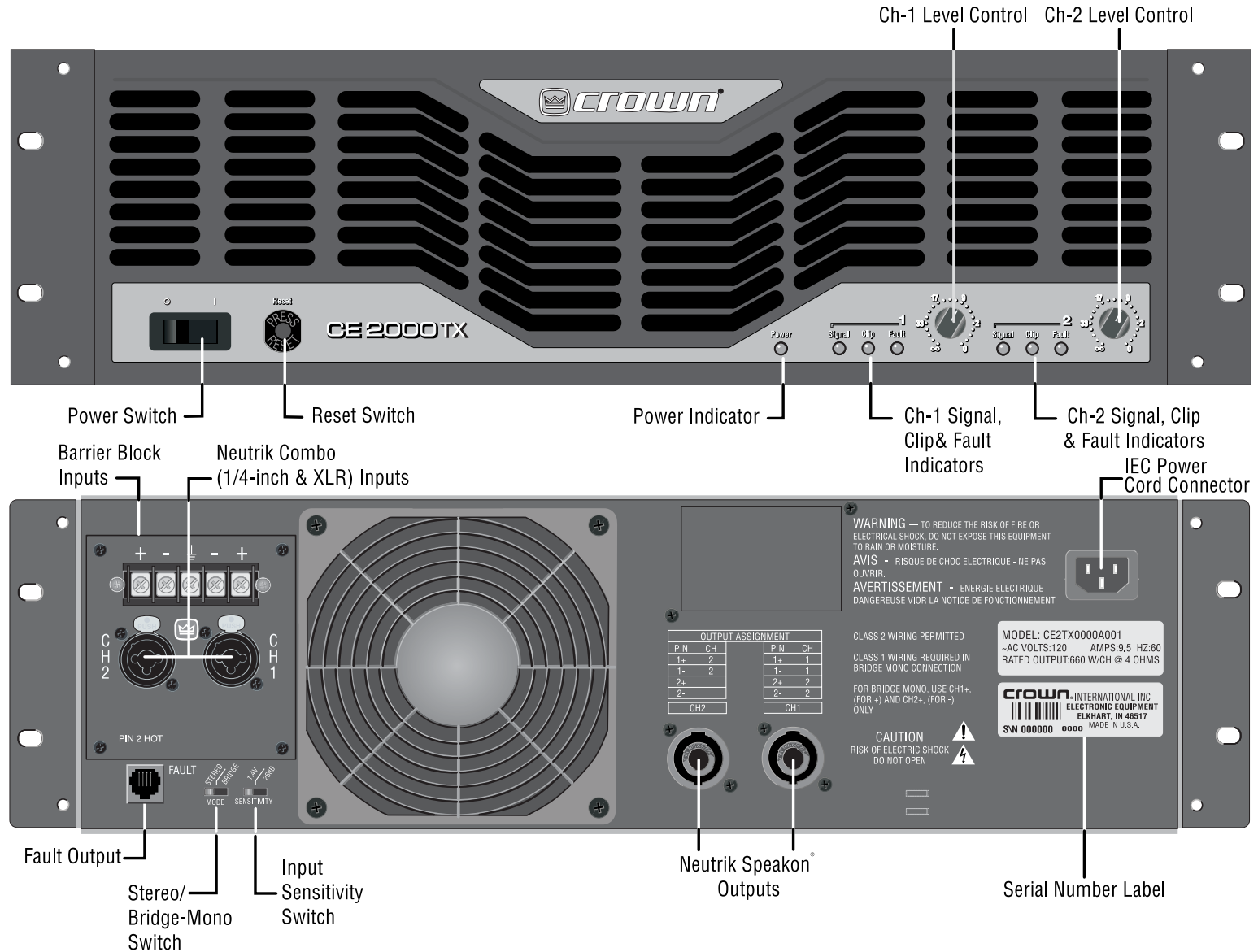
Figure 4.1 Controls, Indicators & Connectors
