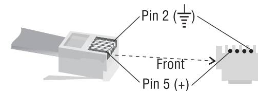
Figure 5.4 RJ-11 Jack Wiring and Pin Assignments
