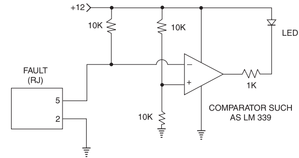
Figure 5.3 Fault Status LED Circuitry
