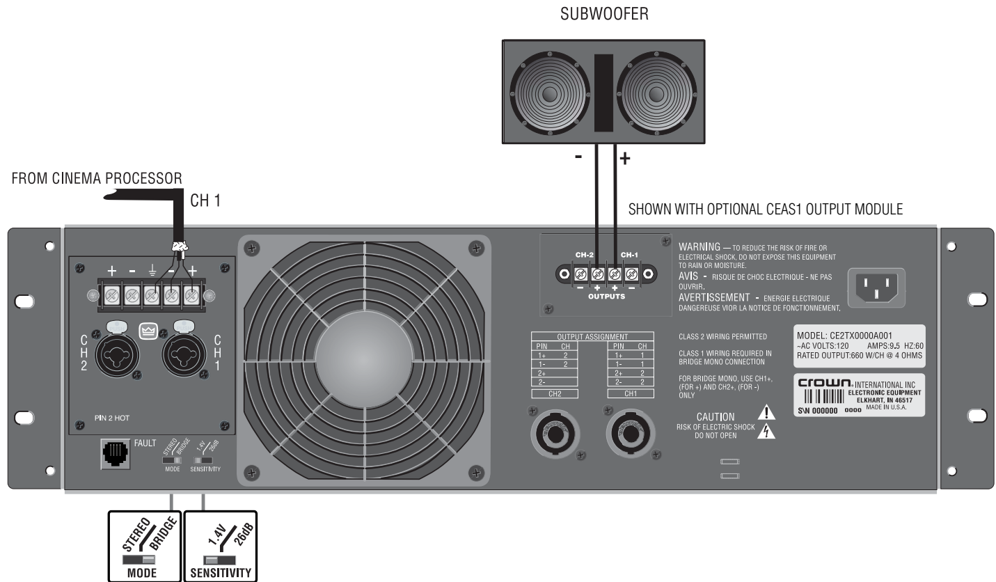
Figure 3.11 Typical System Wiring, Bridge Mono Mode
