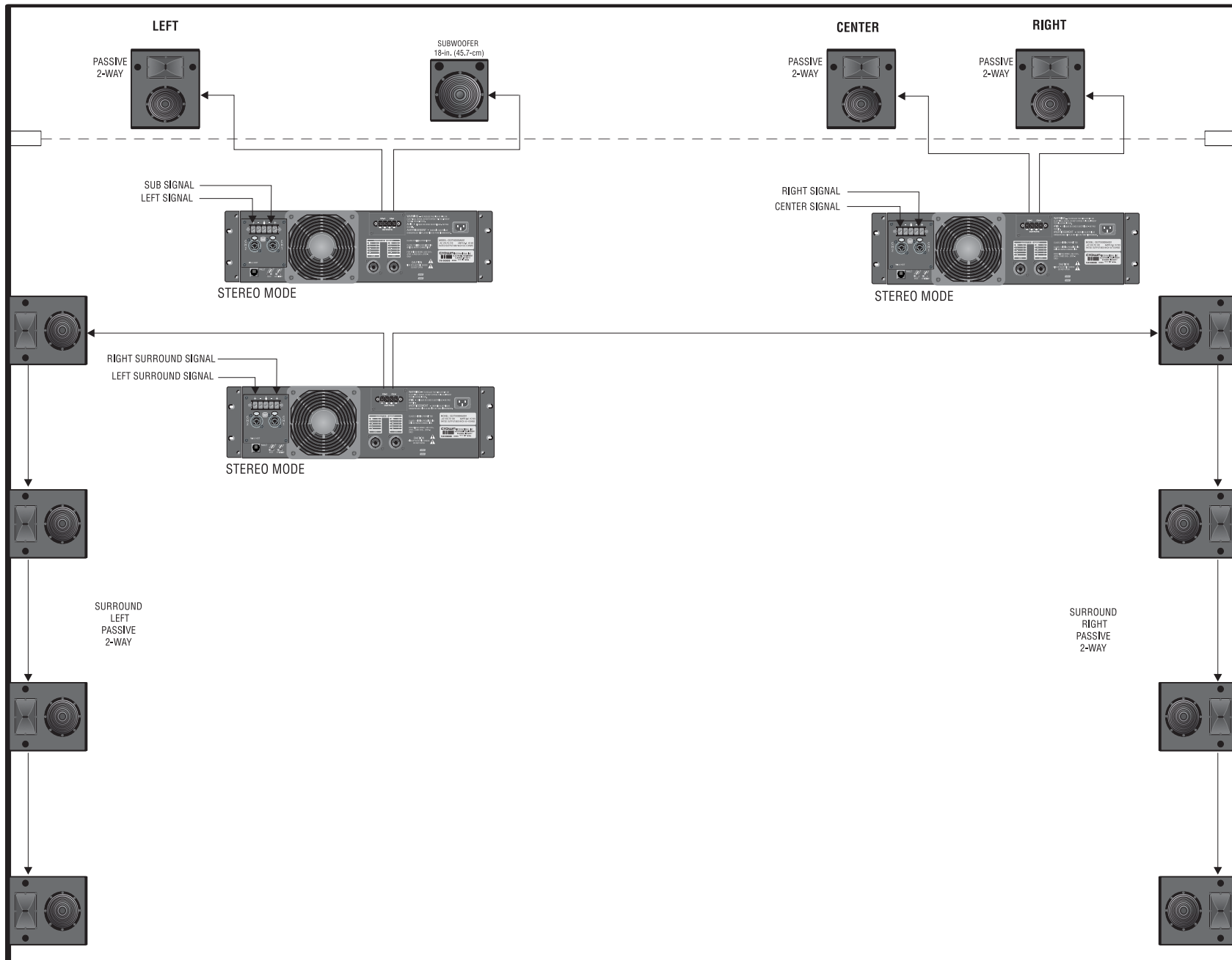
Figure 3.12 Typical Small, Passive System (CE 2000TX Amplifiers Shown with Optional CEAS1 Output Module)
