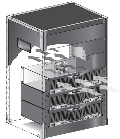
Figure 3.2 Airflow
