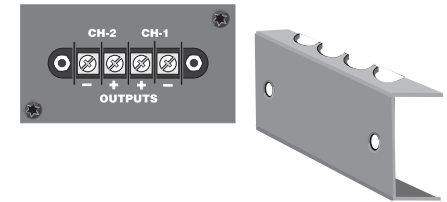
Figure 5.5 Model CEAS1 Barrier Block Output Connectors
