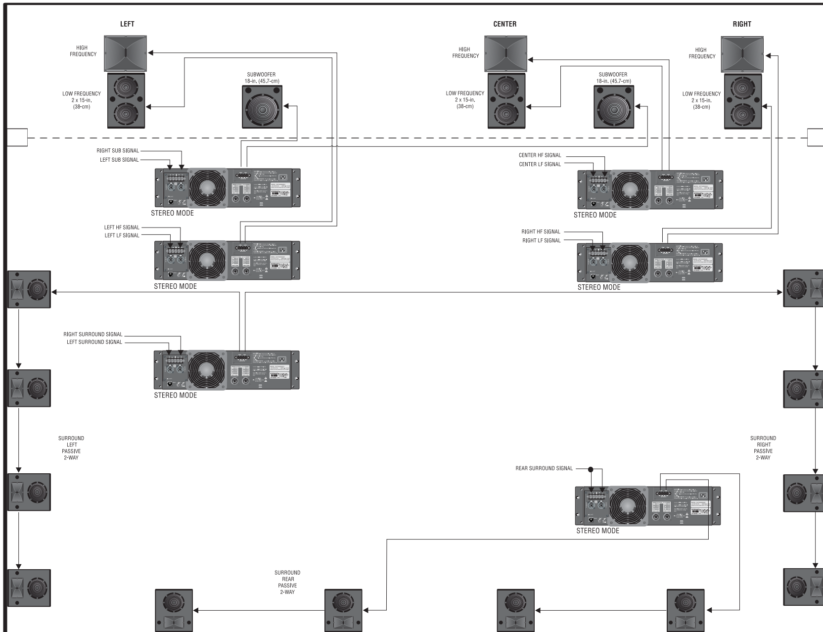
Figure 3.13 Typical Medium 2-Way System (CE 2000TX Amplifiers Shown with Optional CEAS1 Output Module)
