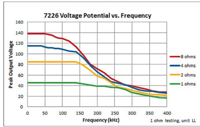
Figure 10.2 – 7226 Voltage Potential vs. Frequency
