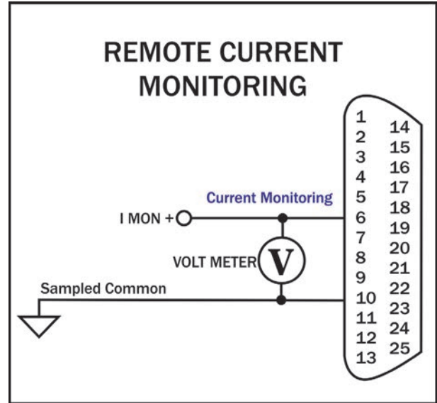
Figure 6.5 – Remote Current Monitoring
