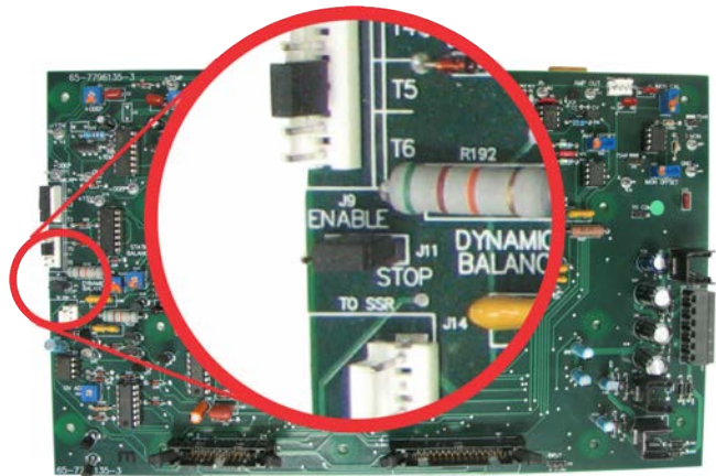
Figure 5.7 – Run Mode/Stop Mode on Power-Up Setting
