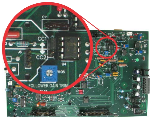
Figure 5.6 – Compensation Setting
