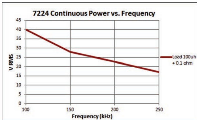
Figure 10.5 – 7224 Continuous Power vs. Frequency
