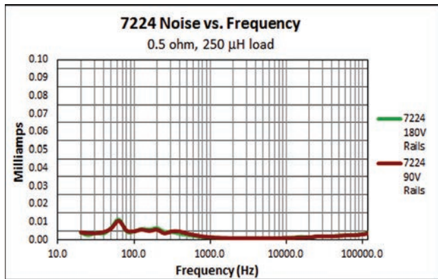
Figure 10.4 – 7224 Noise vs. Frequency
