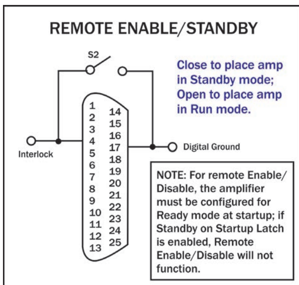
Figure 6.4 – Remote Enable/Standby
