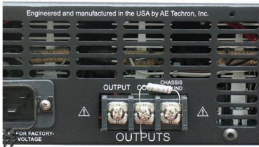
Figure 3.2 – Closeup of the Output Terminal Resistor
