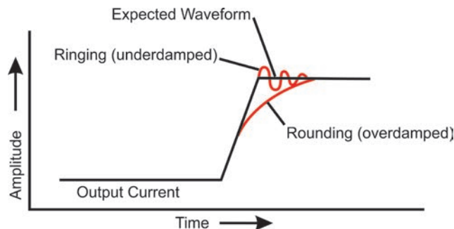
Figure 6.11 – Compensation Effects on Waveform
