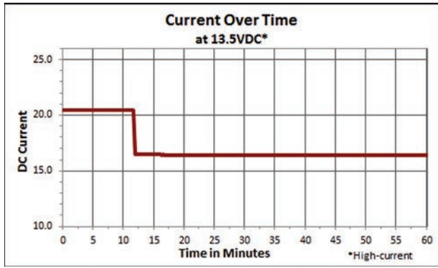
Figure 10.7 – 7224 DC Current Over Time at 13.5 VDC
