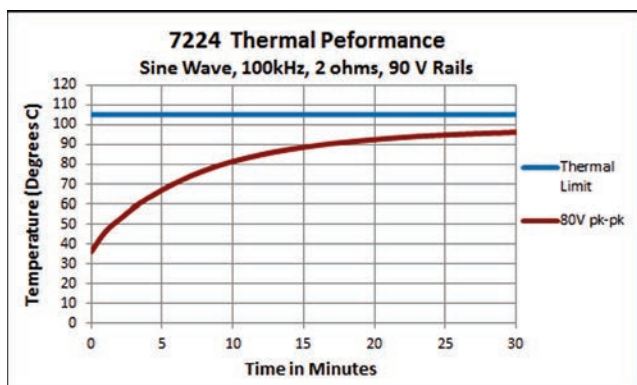
Figure 10.6 – 7224 Thermal Performance
