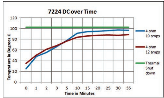
Figure 10.8 – 7224 DC Current Over Time Comparison with 4-ohm Load
