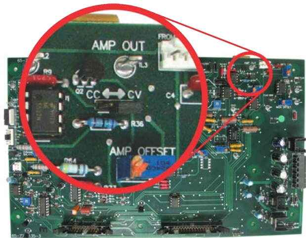
Figure 5.5 – Controlled-Voltage/ Controlled-Current Mode Setting
