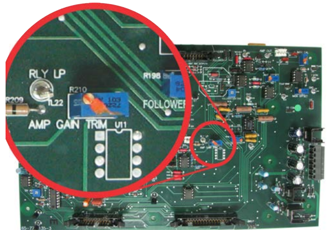
Figure 5.3 – Master/Follower Setting
