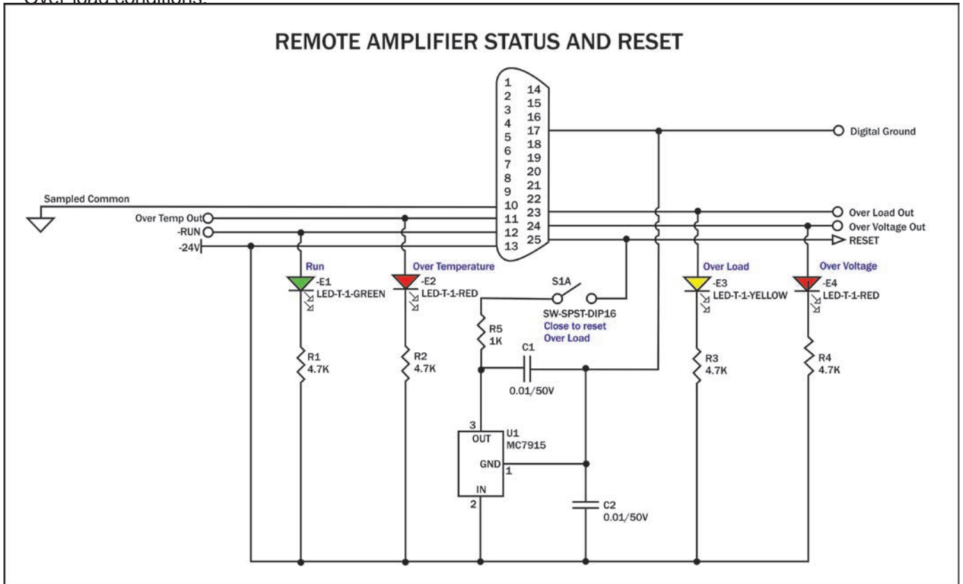
Figure 6.3 – Remote Status and Reset Schematic
