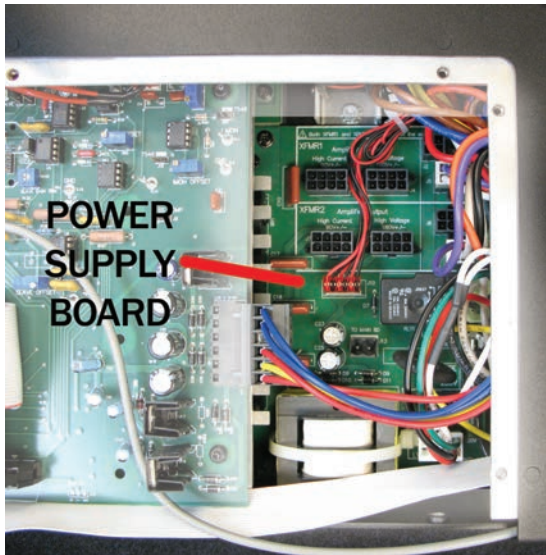
Figure 5.9 – Accessing the Power Supply Board
