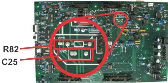
Figure 6.10 – Custom Compensation Location
