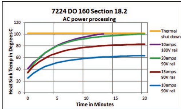
Figure 10.9 – 7224 DO 160 Section 18.2 AC Power Processing
