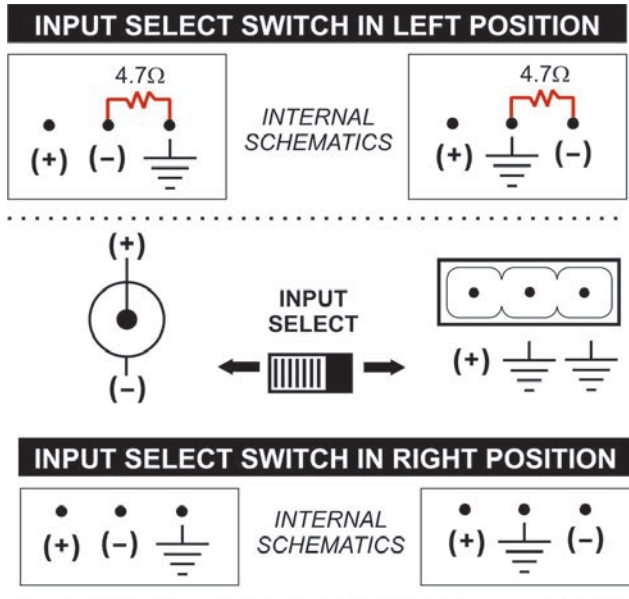
Figure 3.5 – Wiring for Unbalanced or Balanced Input Connector
