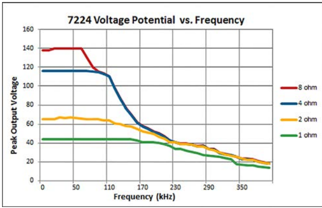
Figure 10.1 – 7224 Voltage Potential vs. Frequency
