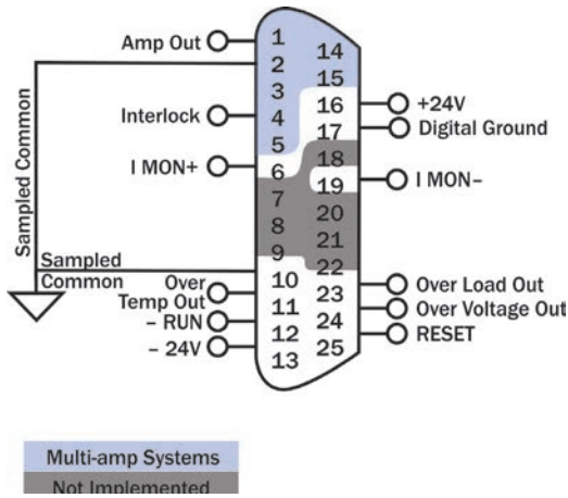
Figure 6.1 – Remote Status and Control Pinouts
