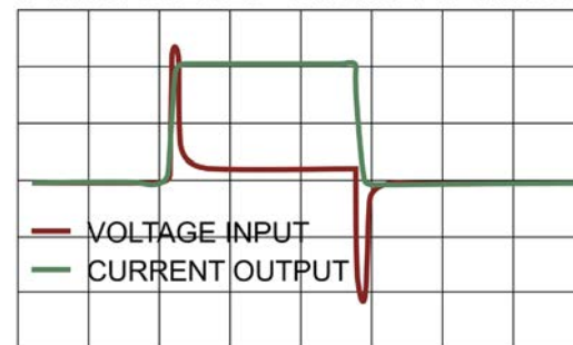
Figure 6.8 – Input to Output Comparison, Controlled-Current Operation
