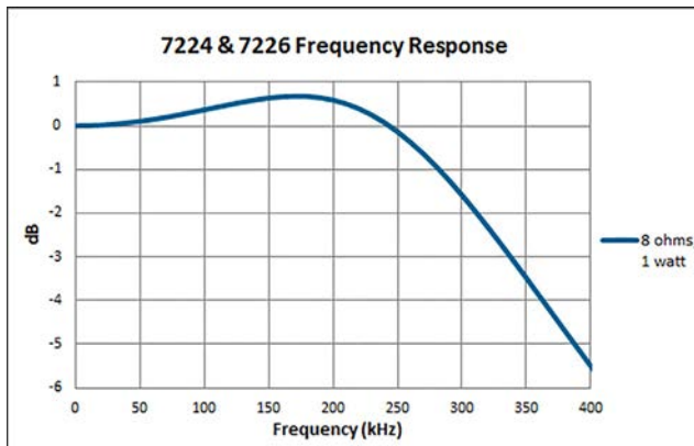
Figure 10.3 – 7224 & 7226 Frequency Response
