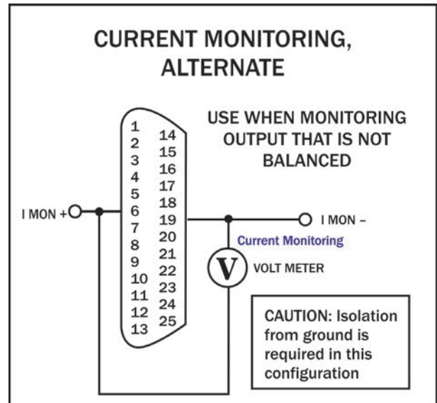
Figure 6.6 – Remote Current Monitoring, Alternate Method
