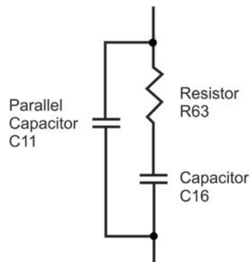
Figure 6.9 – Factory-installed Default RC Network
