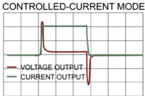
Figure 7.3 – Input to Output Comparison, Controlled-Current Operation
