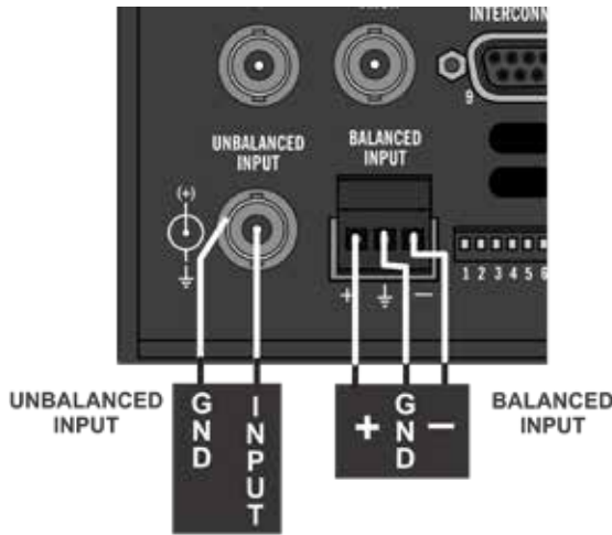
Figure 4.4 – Wiring for Unbalanced or Balanced Input Connector
