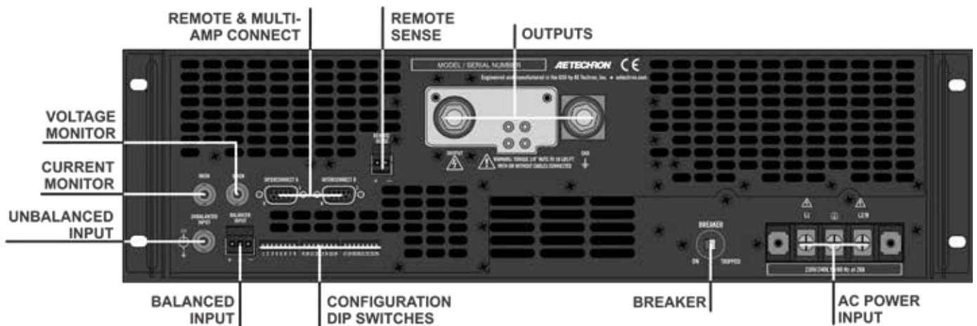
Figure 5.2 – Back Panel Controls and Connectors
