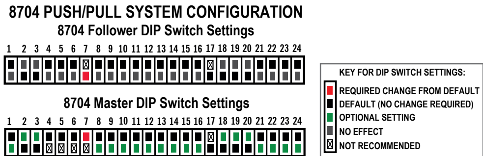
Figure 7.12 – Required DIP switch settings for Push/Pull amplifiers
